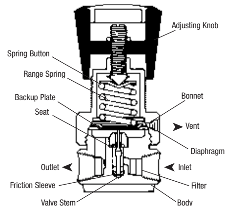
Fig. 1 Single-stage regulator.
